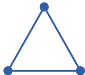
P_1 Lagrange
