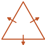
RT_0
