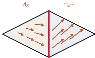
(a) a Raviart–Thomas field
