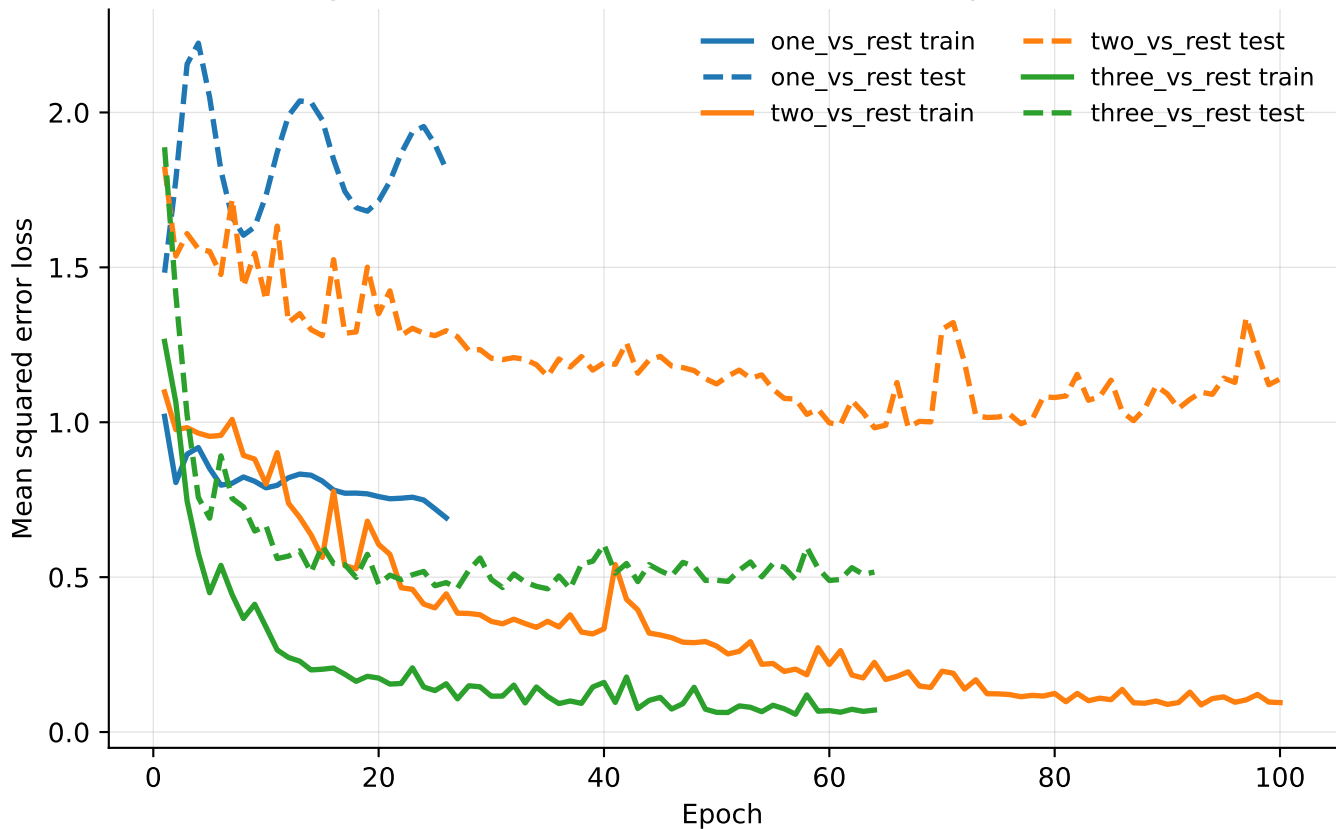
Training and test loss for best fused attention quickstart model
