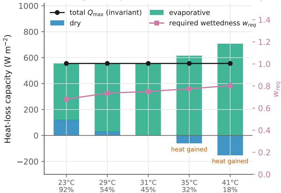
(b) Along the isopleth the routes trade off exactly
