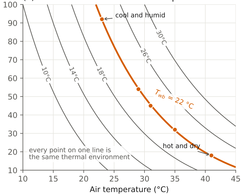
(a) Lines of constant wet-bulb temperature
