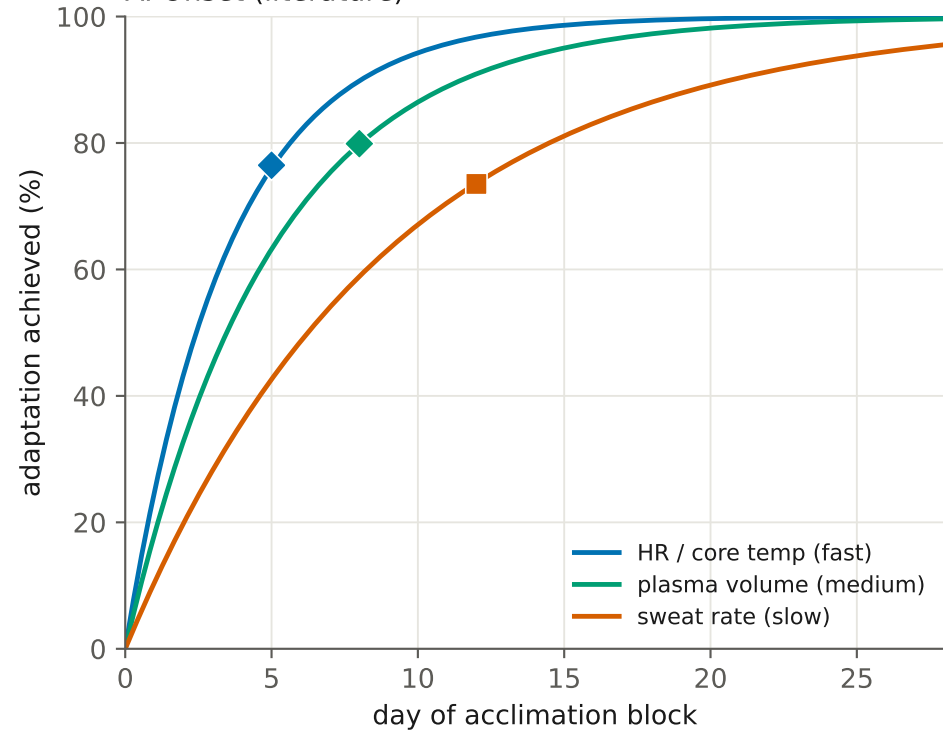
A. Onset (literature)
