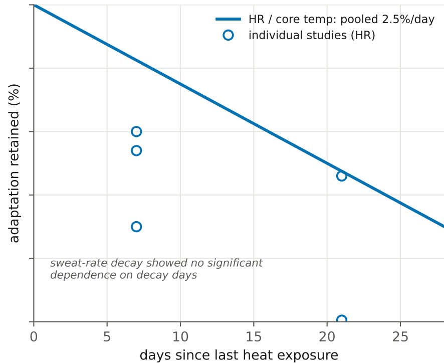
B. Decay (literature)
