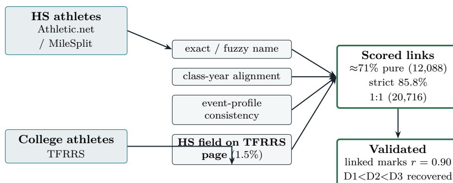
Figure 11: Probabilistic HS→college linkage. No exact key exists; a scored combination of name, year and event profile reaches ~71% precision, and TFRRS athlete pages carry a literal High School field (1.5% of pages) that opens a path to a real crosswalk by crawling those pages directly.
