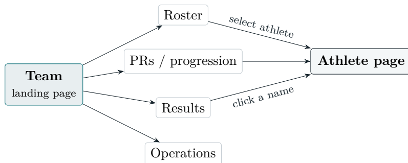
Figure 6: The Team tab. The athlete page is secondary: reached from the roster, the PR / progression boards, or any result line — all three converge on the same object. Operations stays team-level.
