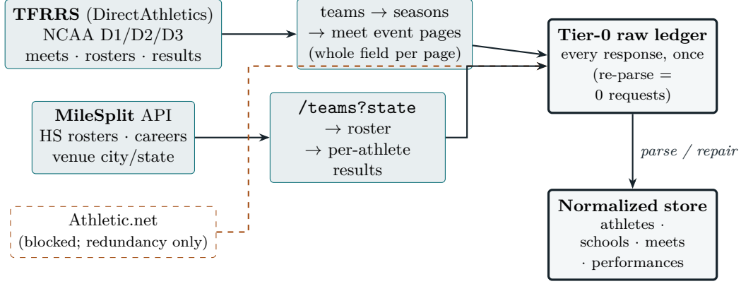
Figure 2: Roster/meet/team sourcing. Every response tees to a raw ledger before parsing, so a parser fix replays at zero request cost. Athletic.net (dashed) is demoted to redundancy.
