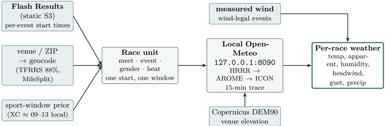
Figure 3: Weather + elevation per race , not per meet. The 11 am women’s JV and the 3 pm men’s varsity get different windows. Wind for sprints comes measured from the results themselves.
