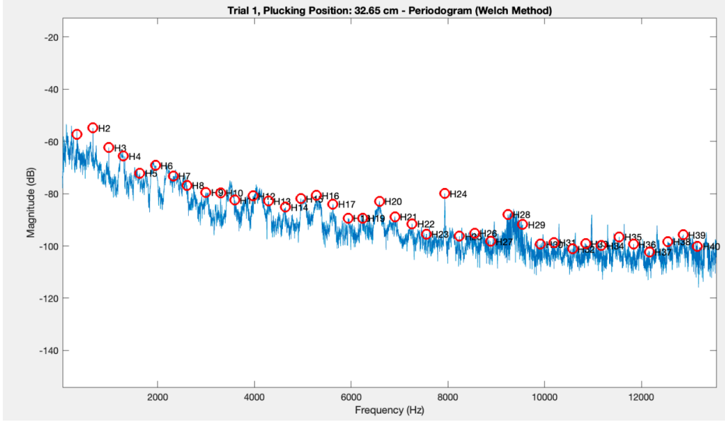
Figure 6: Example of frequency-domain data showing harmonic peaks
