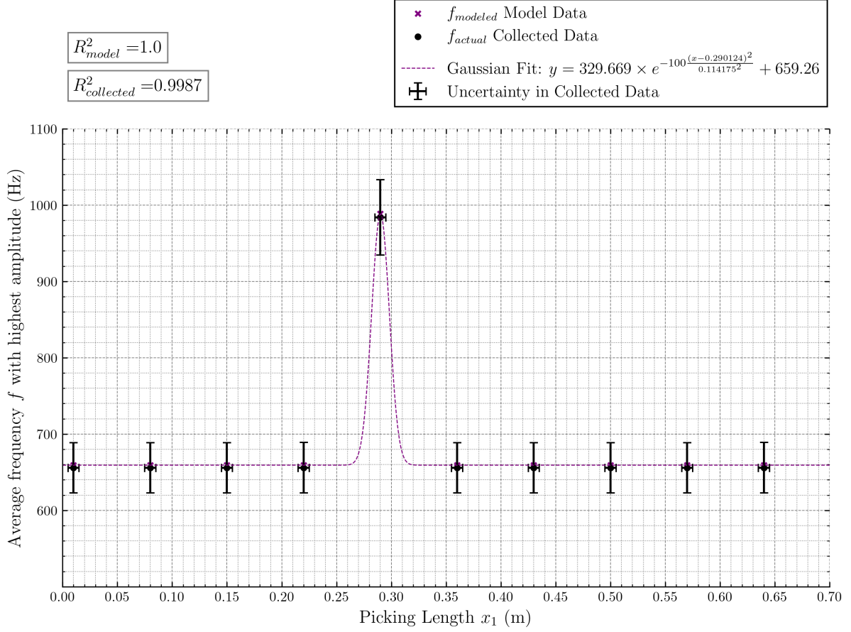
Figure 5: Comparison between \bar{f}_{actual} and \bar{f}_{modeled} with Gaussian trendline
