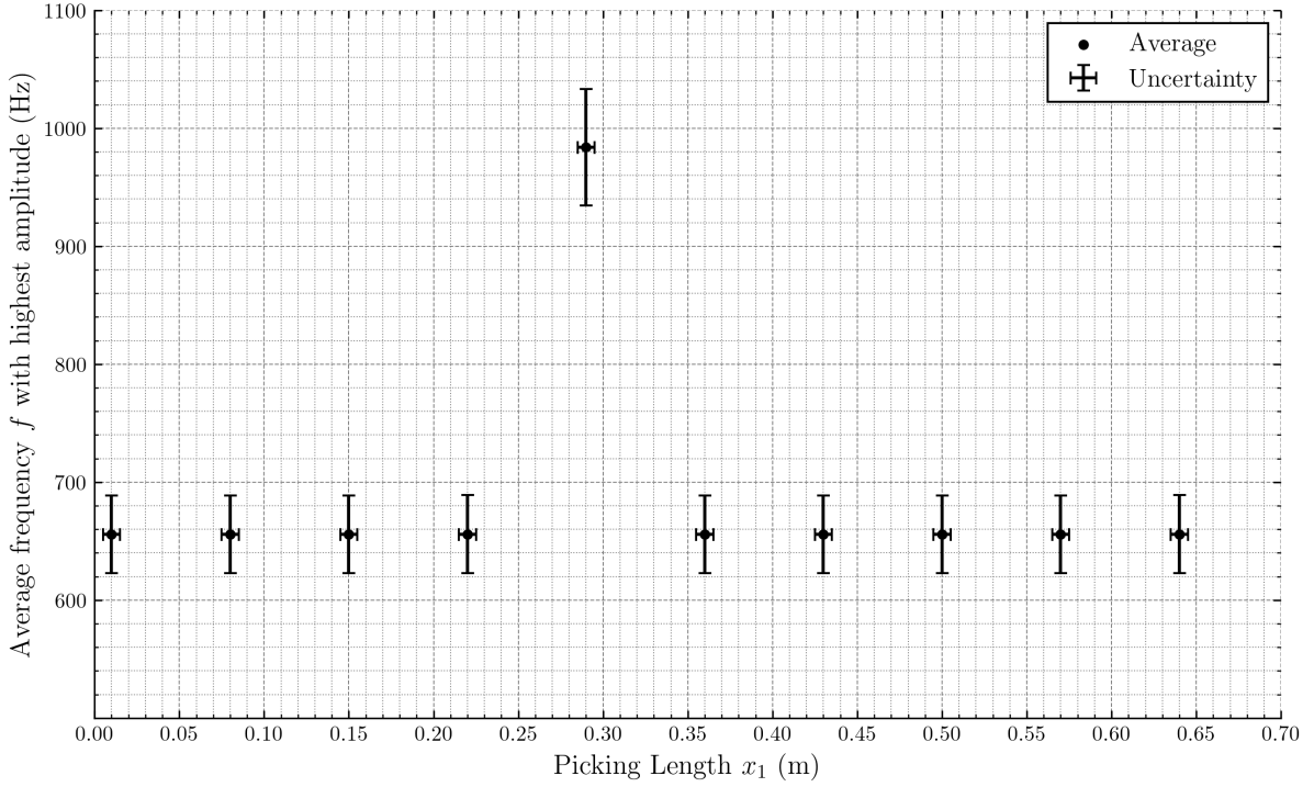
Figure 4: Graph of picking length x_1 against average frequency \bar{f}
