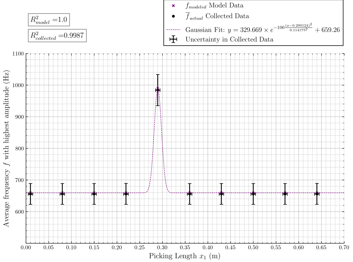
Figure 5: Comparison between \bar{f}_{\text{actual}} and f_{\text{modeled}} with Gaussian trendline
