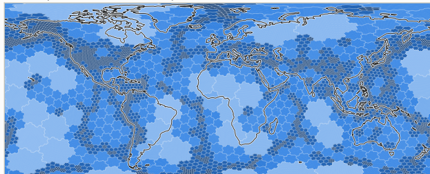
Earthquakes: tree, best partition: 5,993 bins
