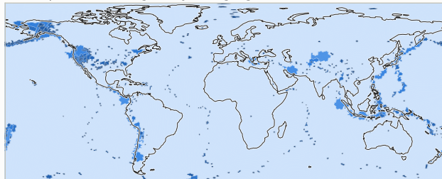
Earthquakes: then greedy merging: 539 bins
