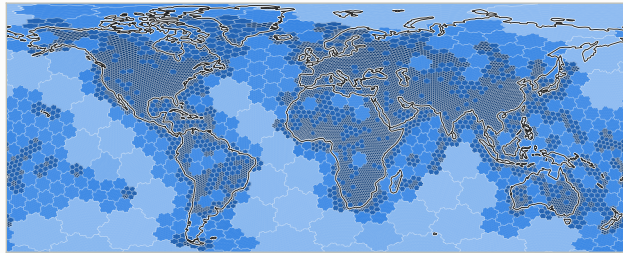
News events: tree, best partition: 9,668 bins
