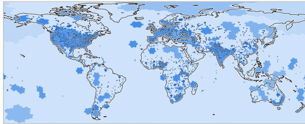
News events: then greedy merging: 1,457 bins
