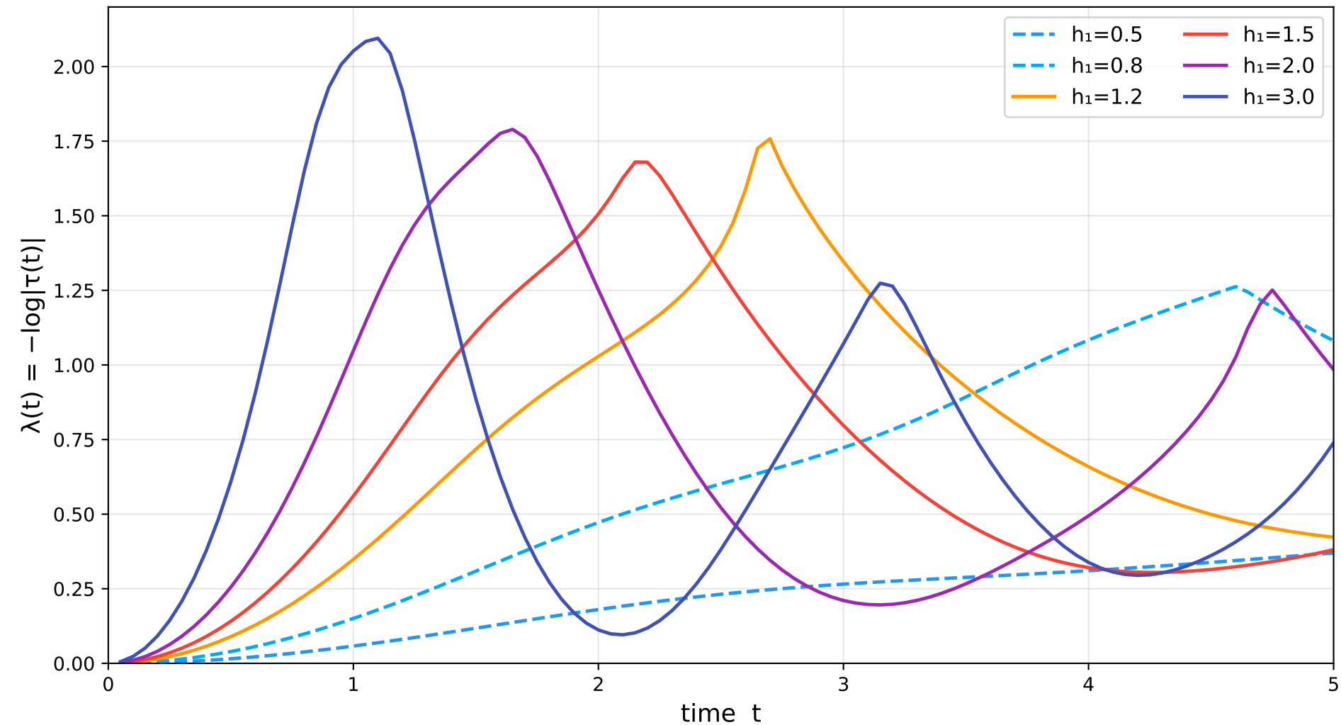
Loschmidt Echo Rate (TFIM, J=1.0 , \chi_{\text{max}}=40 , dt=0.05 ) Dashed: h_1 < 1 (ordered), Solid: h_1 > 1 (cusps = Dynamical Phase Transitions)
