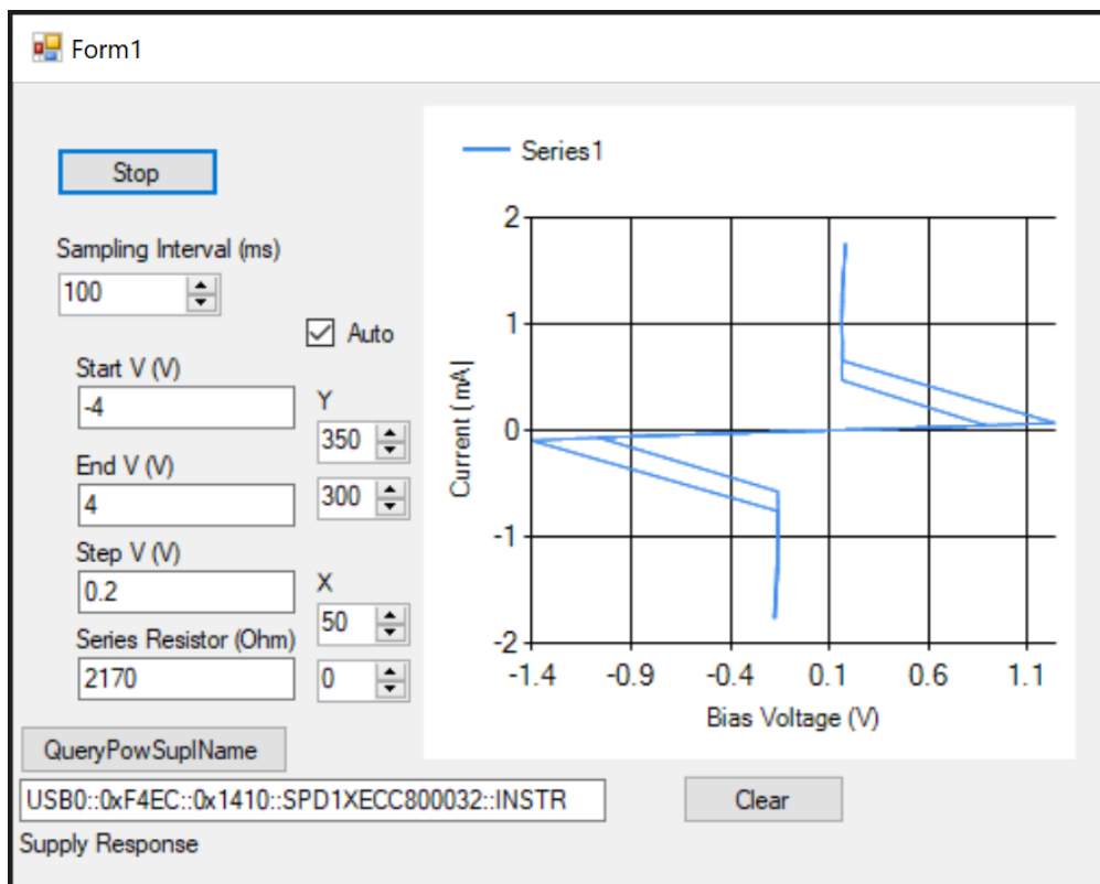
Figure 3: Task 2: I(V) Curve Screenshot
