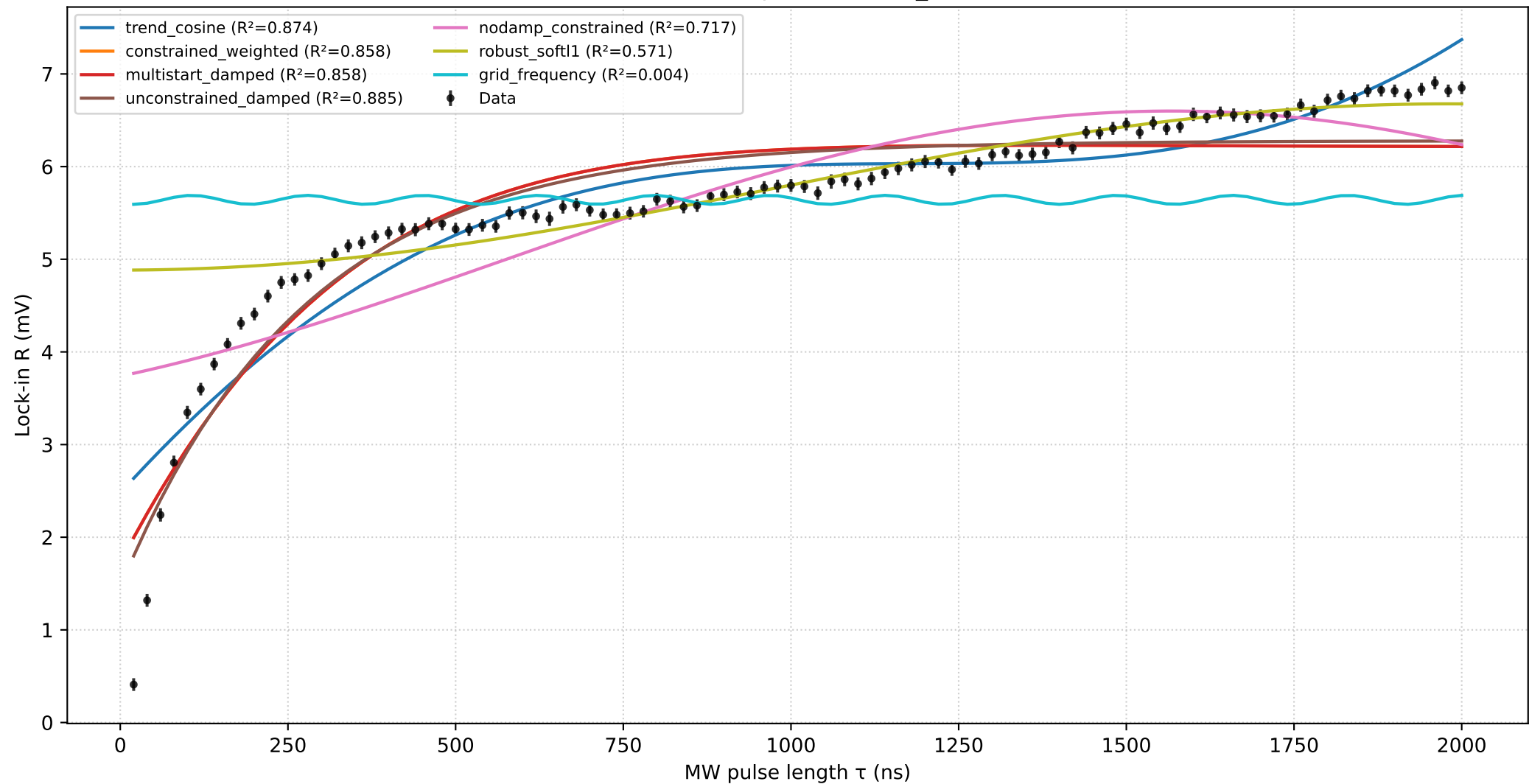
Rabi Method Comparison: Rabi_Corrected
