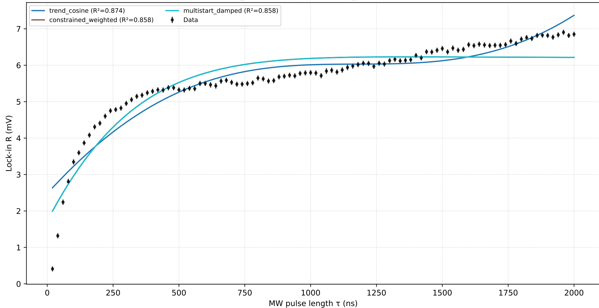
Rabi Top-3 Methods: Rabi_Corrected | Best=trend_cosine ( R^2=0.874 , cycles=0.50)
