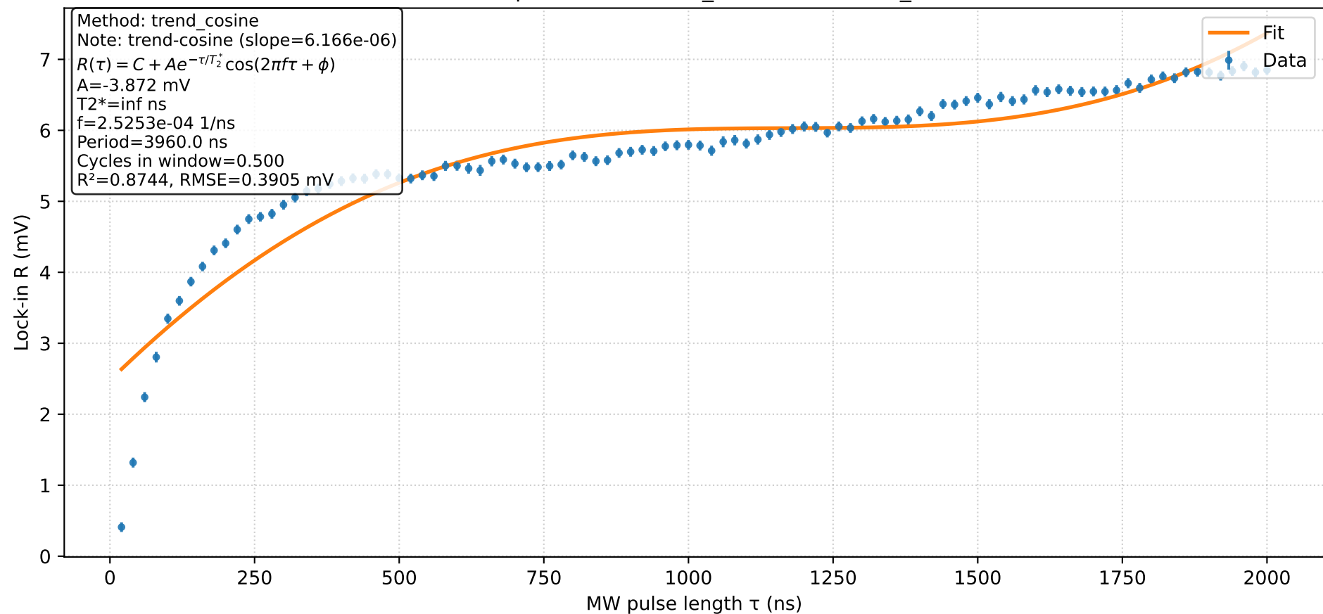
Rabi Fit Improvement: Rabi_Corrected (trend_cosine)
