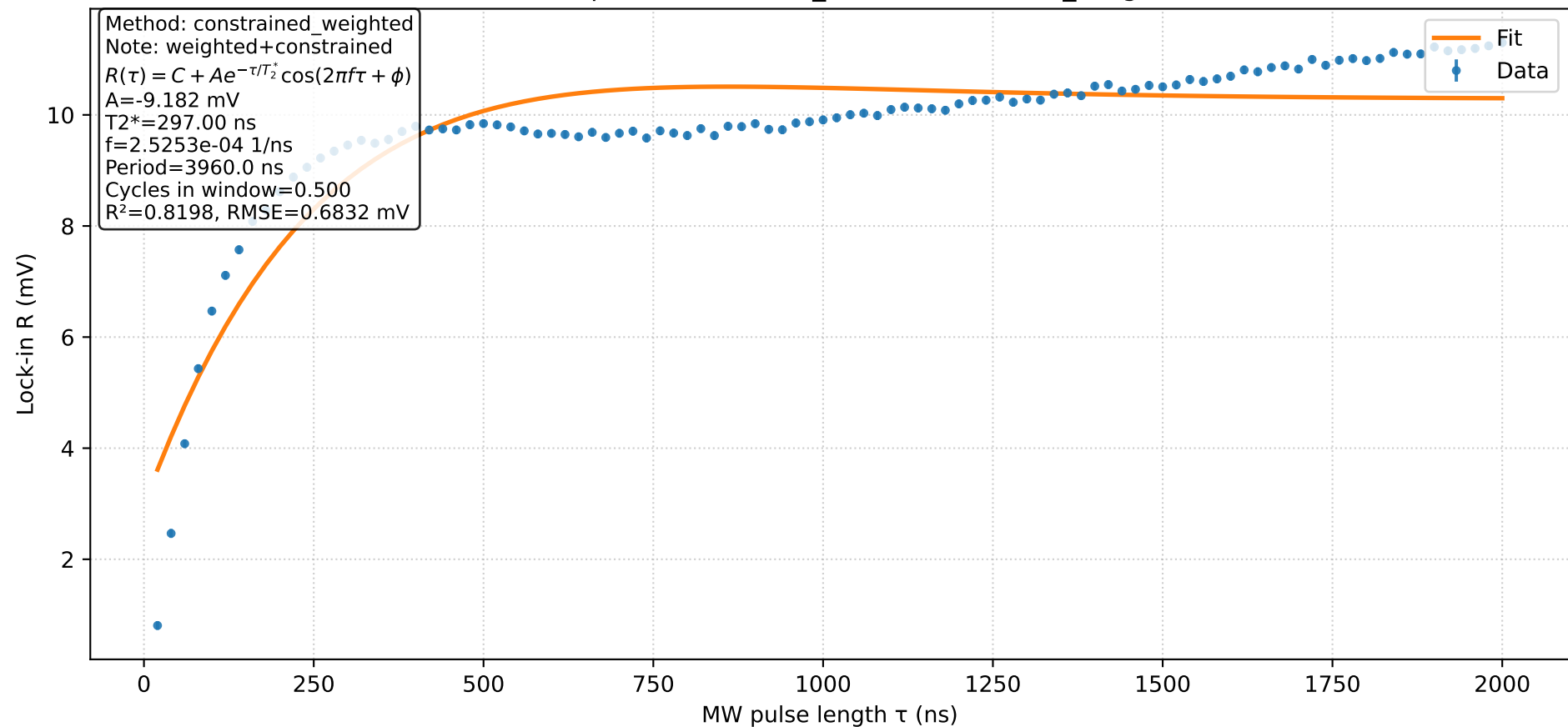
Rabi Fit Improvement: Rabi_tau1 (constrained_weighted)
