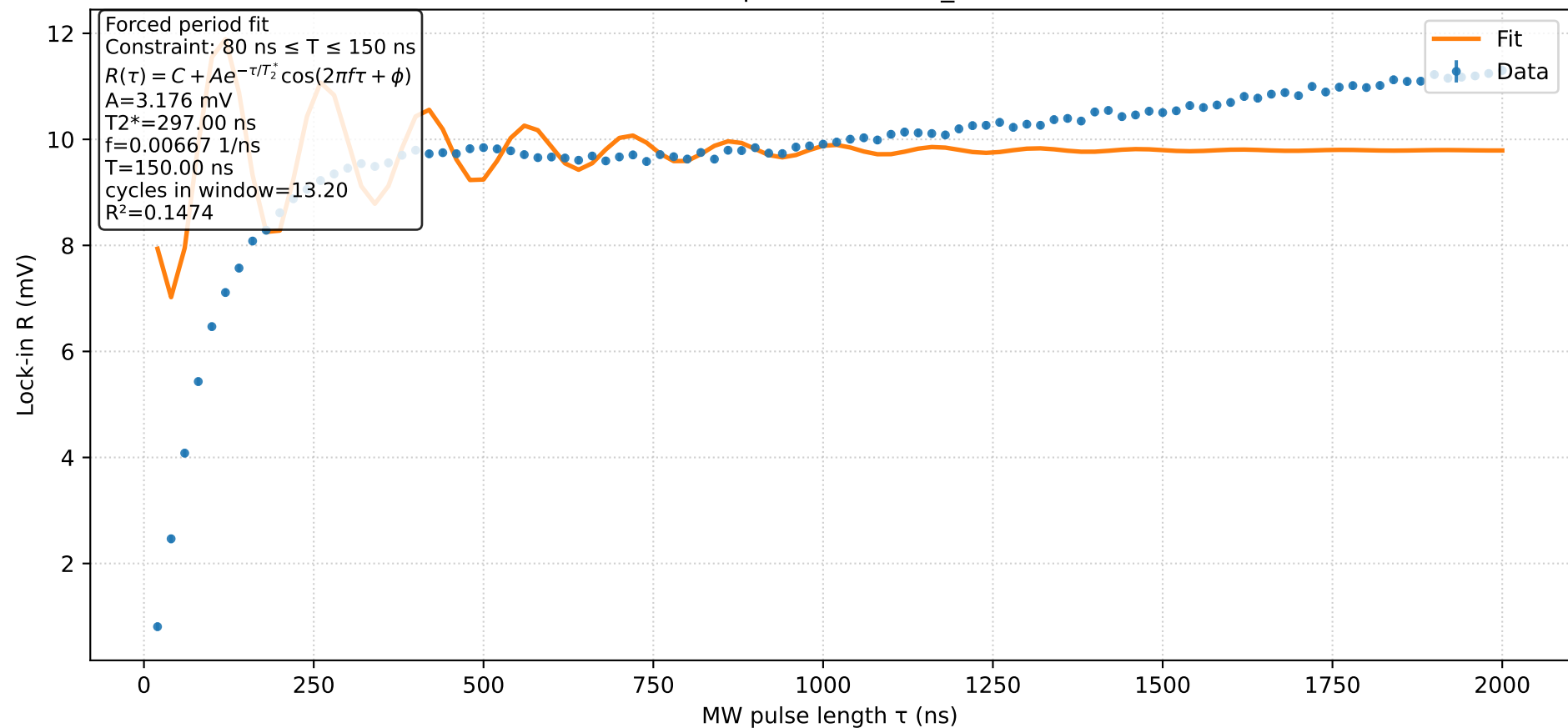
Rabi forced-period fit (Rabi_tau1.csv)
