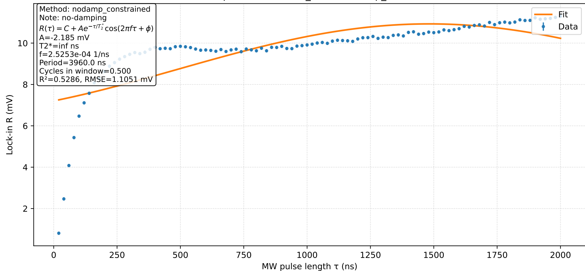
Rabi Fit Improvement: Rabi_tau1 (nodamp_constrained)
