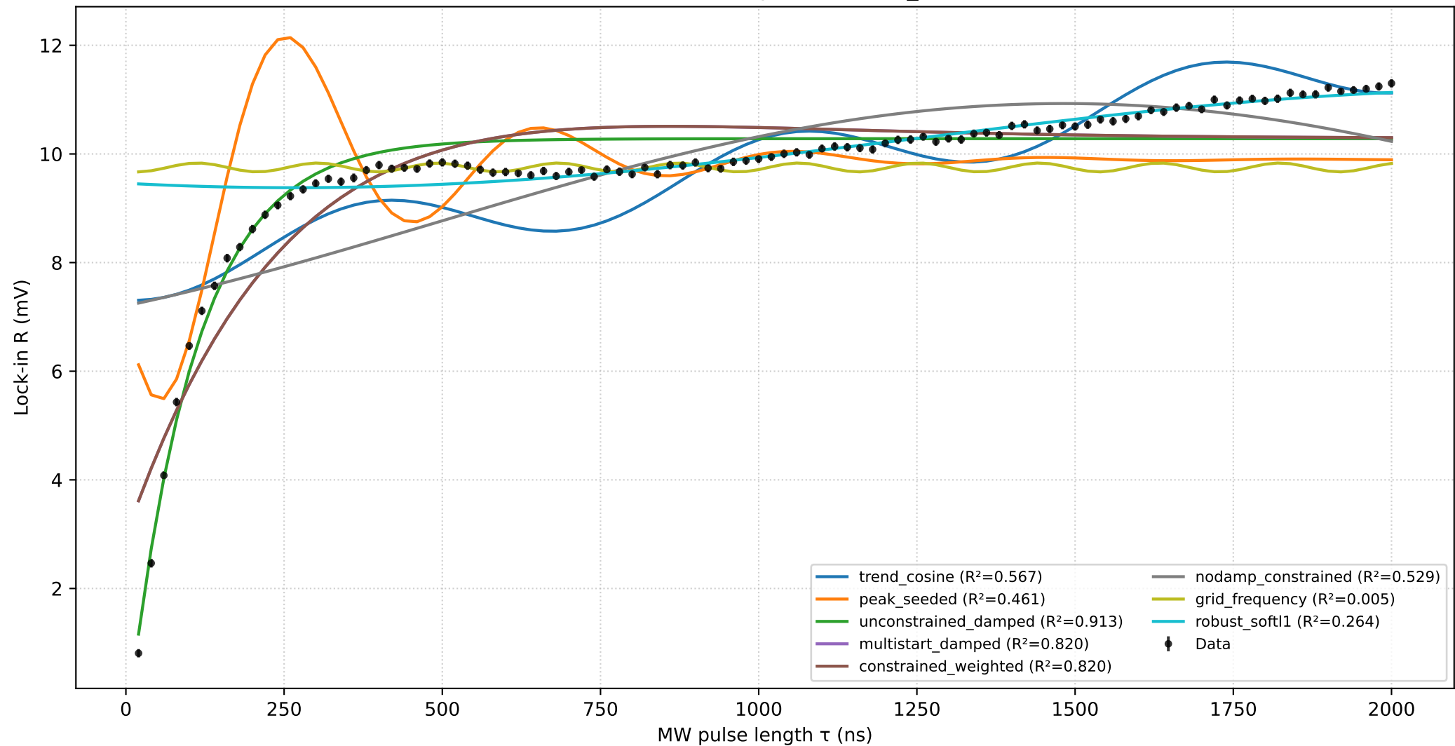
Rabi Method Comparison: Rabi_tau1
