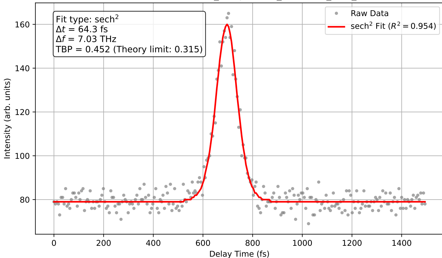
Autocorrelation: autocorr_comp+TeO2_extended_65fs_sech2
