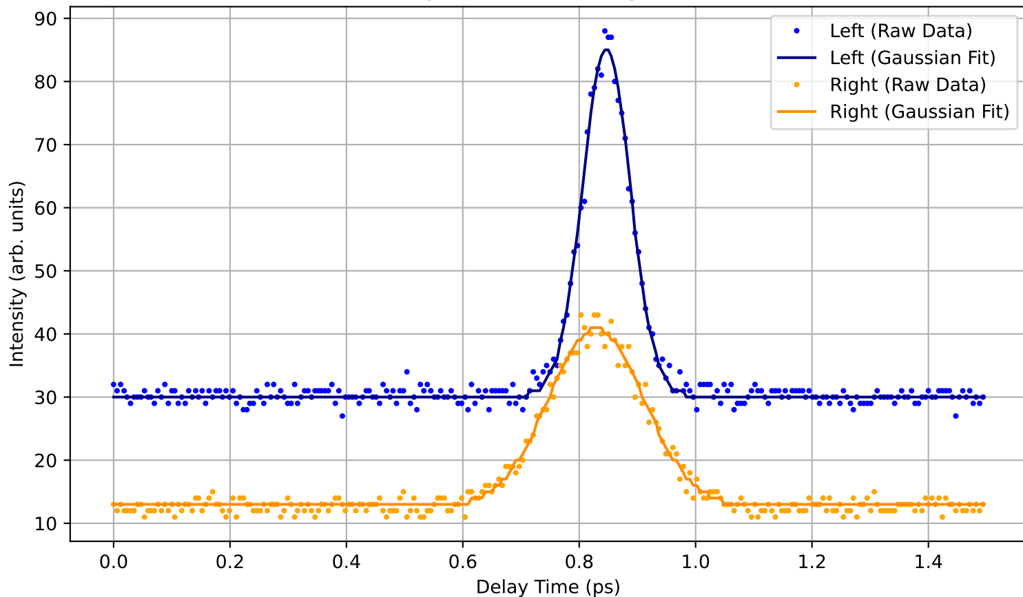
1cm Glass Dispersion (Left vs Right) - Gaussian Fit
