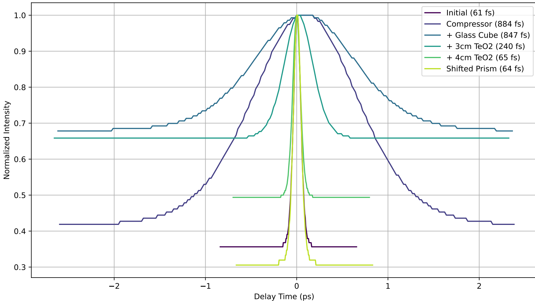
Pulse Compression Evolution (sech 2 Fits - Normalized & Centered)
