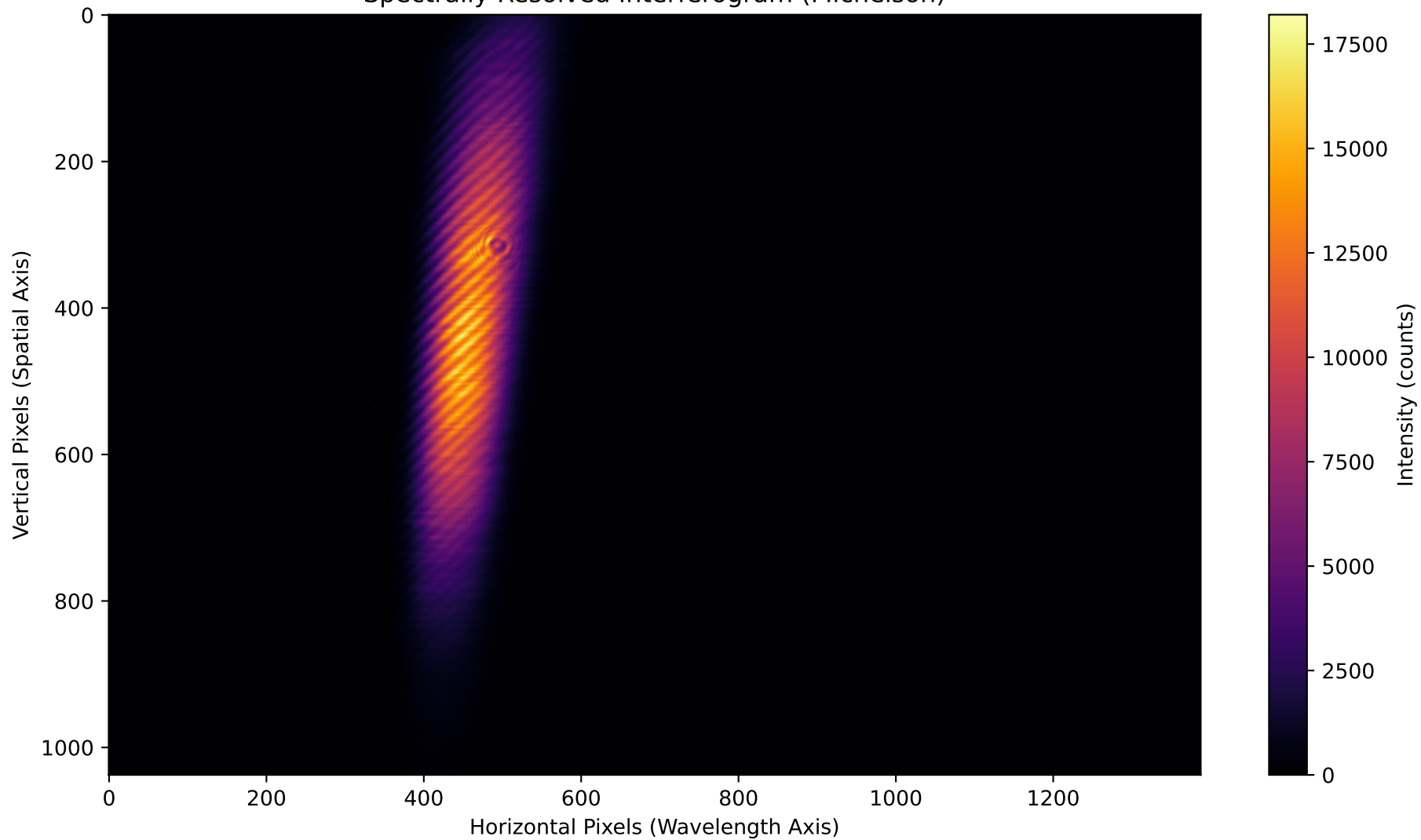
Spectrally Resolved Interferogram (Michelson)
