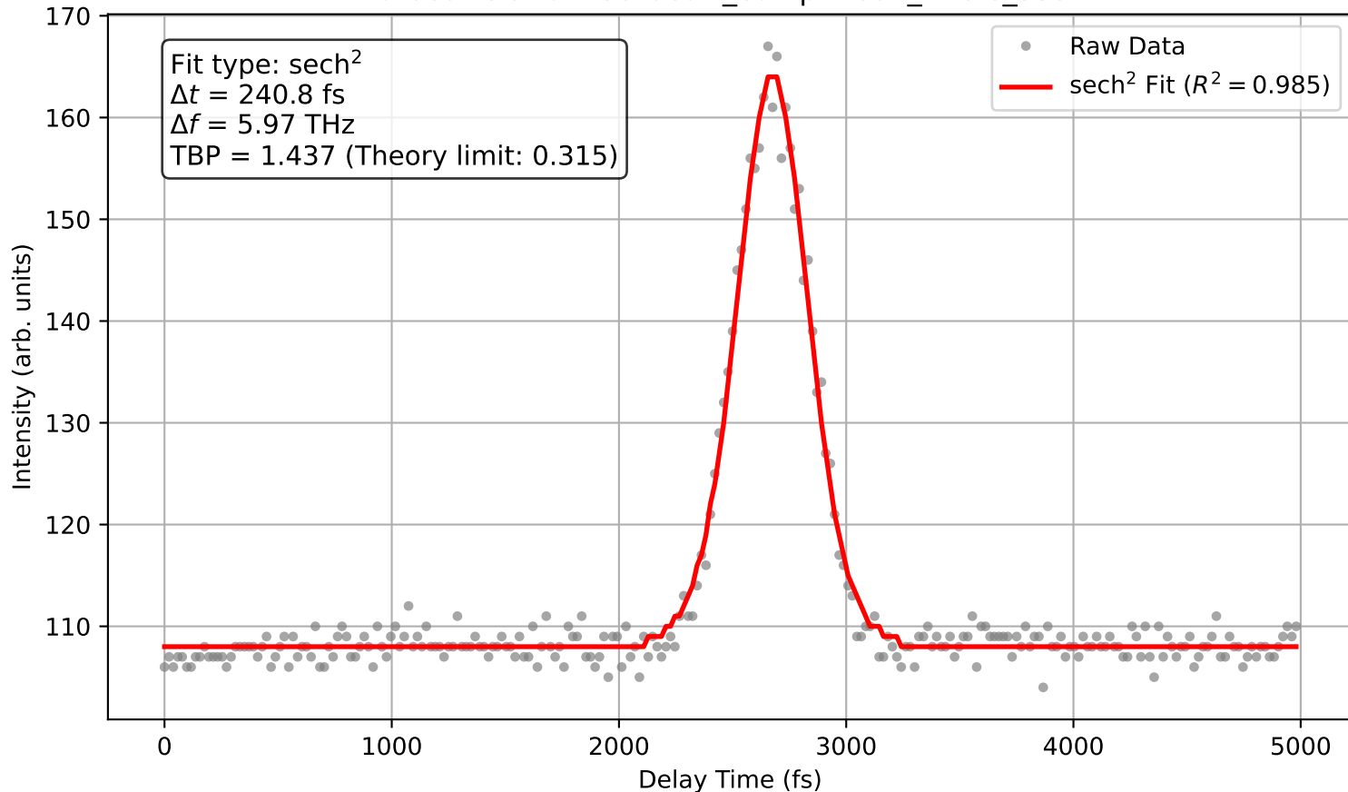
Autocorrelation: autocorr_comp+teo2_240fs_sech2
