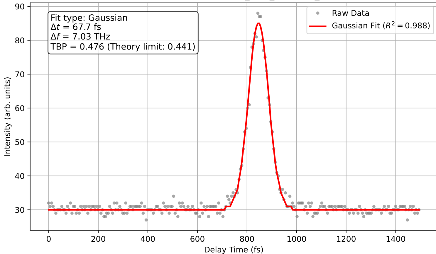
Autocorrelation: autocorr1_68fs_leftpulse_gauss
