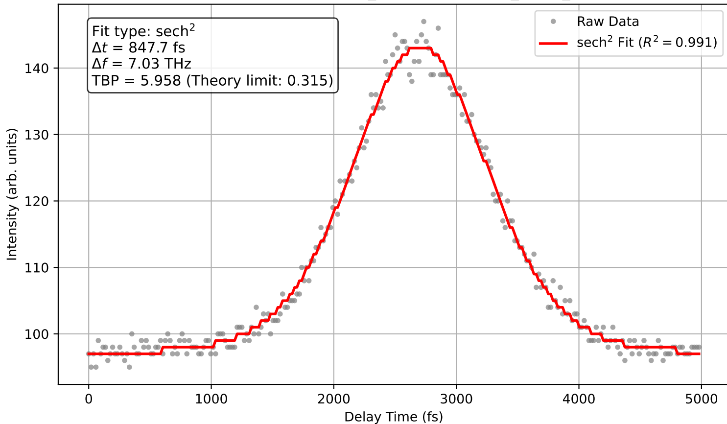
Autocorrelation: autocorr_comp+glasscube_847fs_sech2
