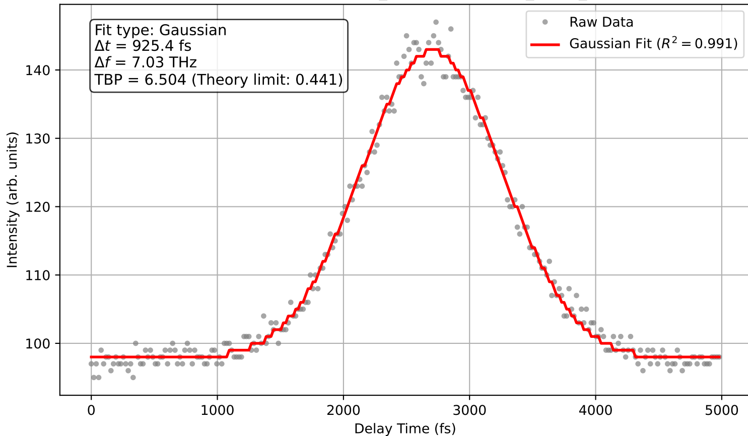
Autocorrelation: autocorr_comp+glasscube_941fs_gauss
