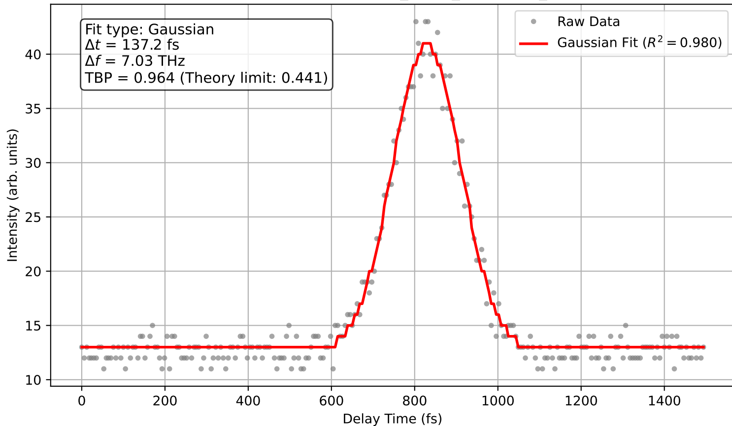
Autocorrelation: autocorr1_138fs_rightpulse_gauss
