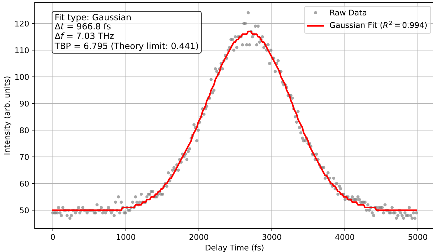
Autocorrelation: autocorr_comp_979fs_gauss
