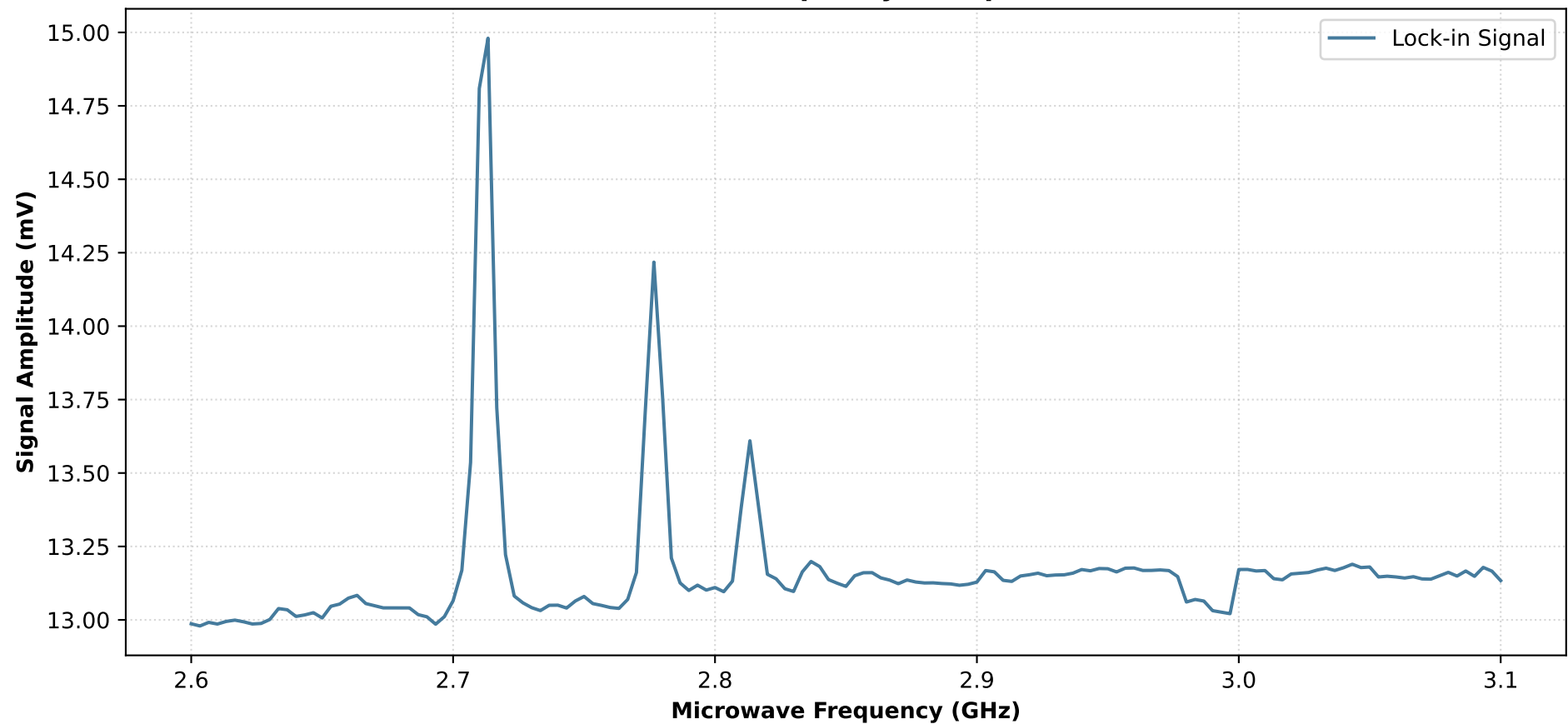
CW frequency sweep
