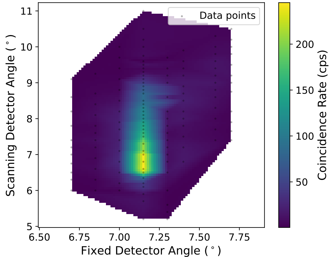
Correlated Coincidence Distribution
