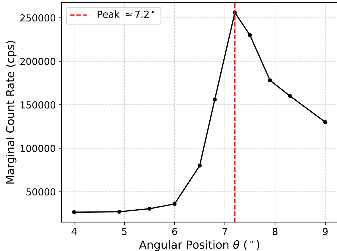
Single-Photon Intensity Distribution
