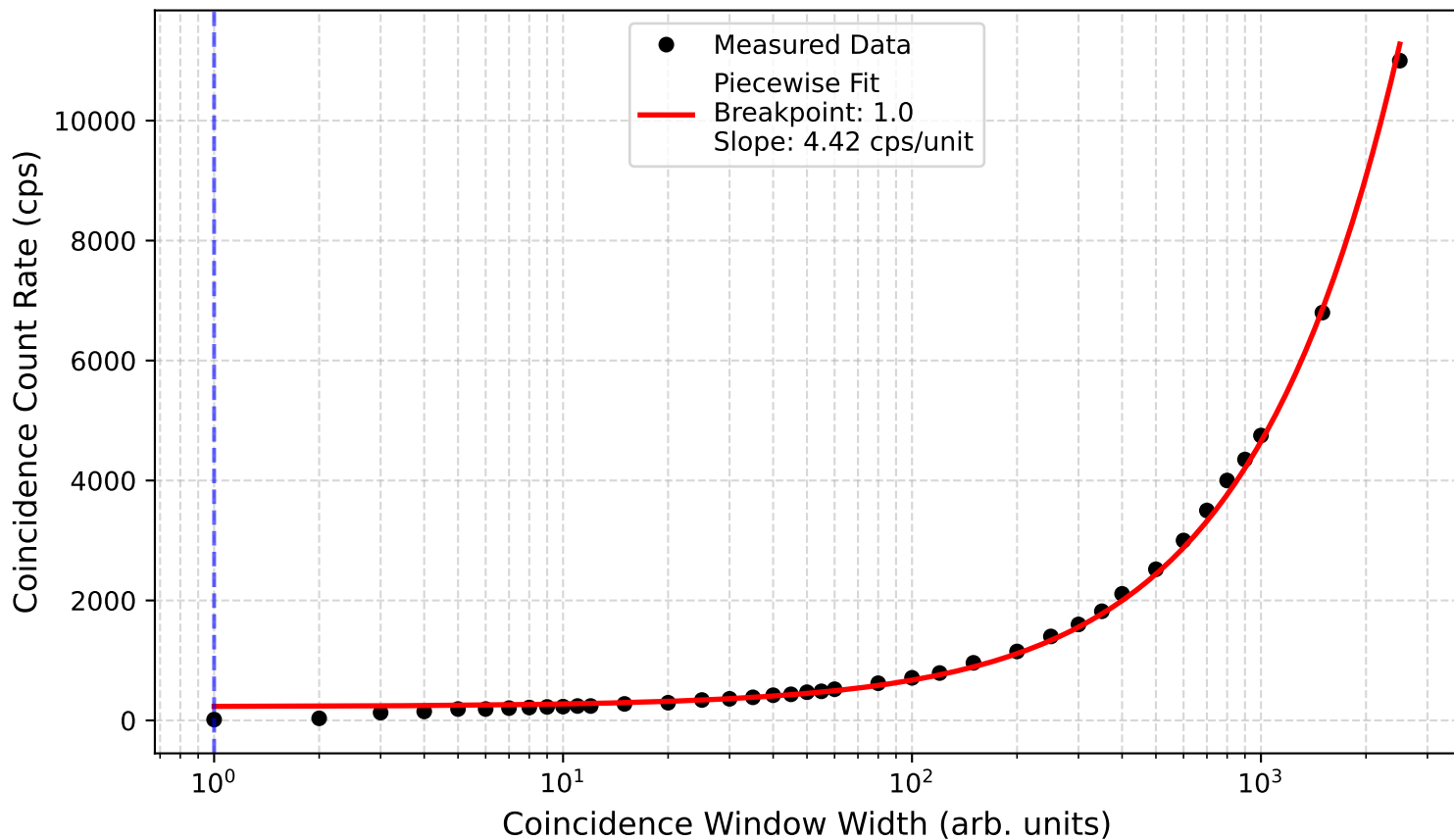
Task 5: Coincidence Rate vs. Window Width
