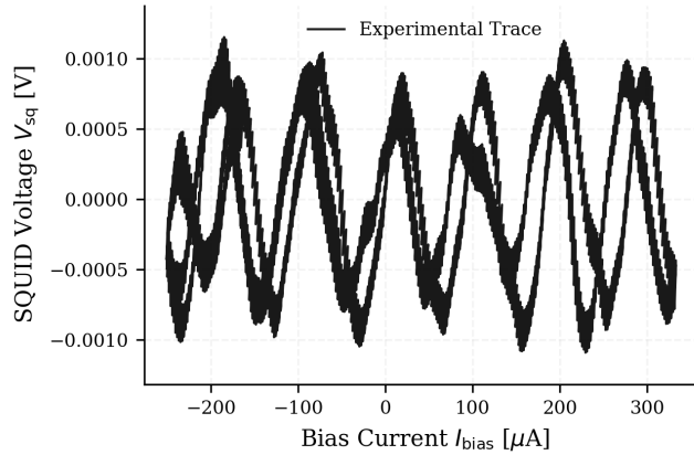
Fig 2: SQUID I-V characteristics under varying magnetic flux.
