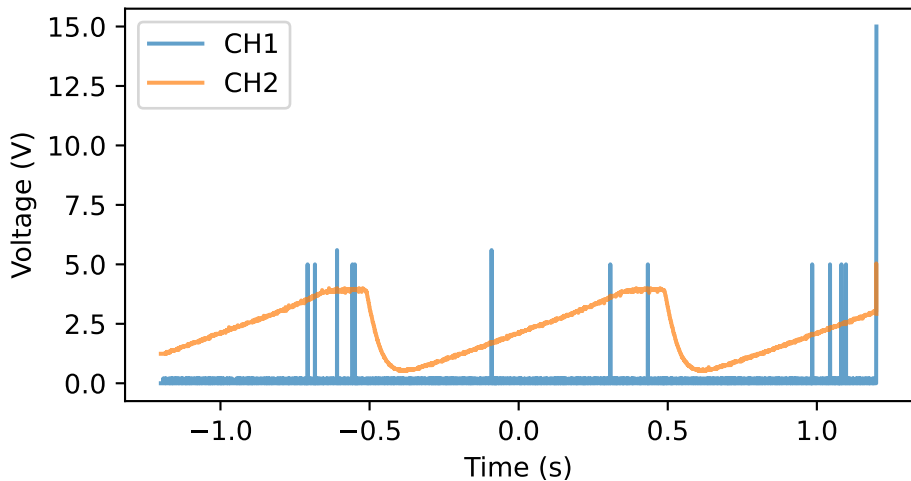
Oscilloscope (NewFile5.csv)
