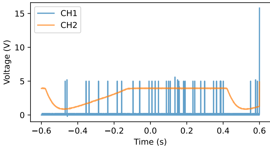
Oscilloscope (NewFile6.csv)
