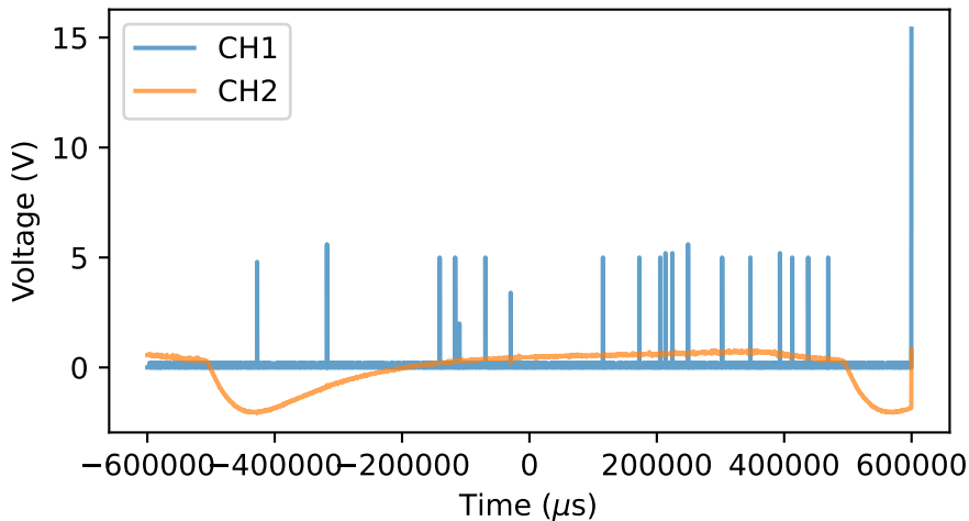
Oscilloscope Sweep (NewFile2.csv)
