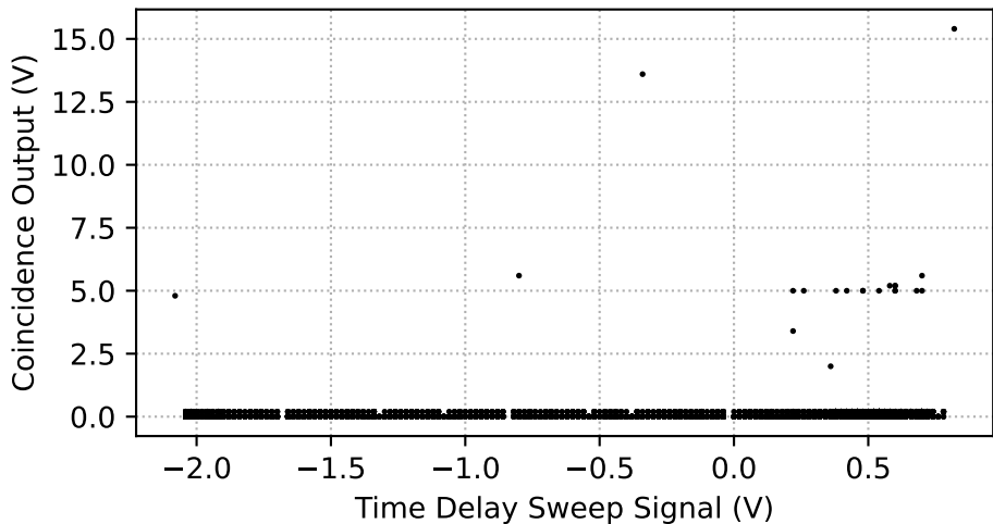
Convolution Profile - Short (230 ns)
