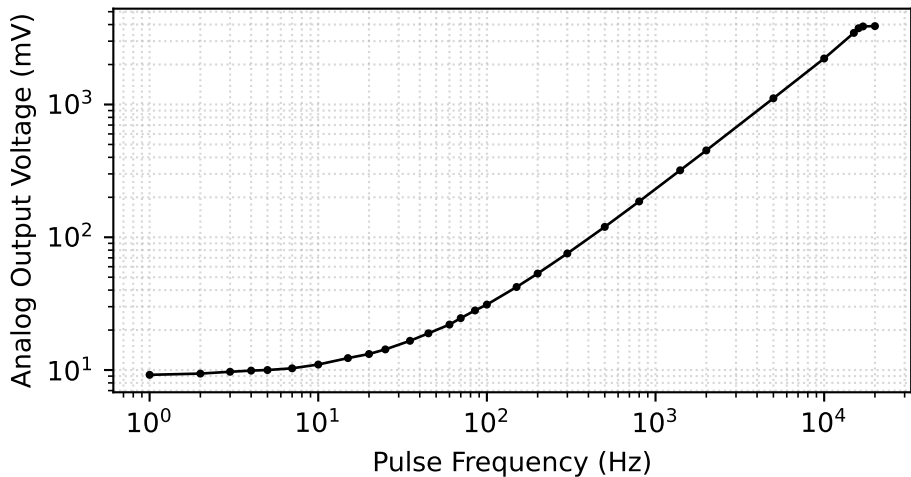
Counter Calibration (230ns pulse)
