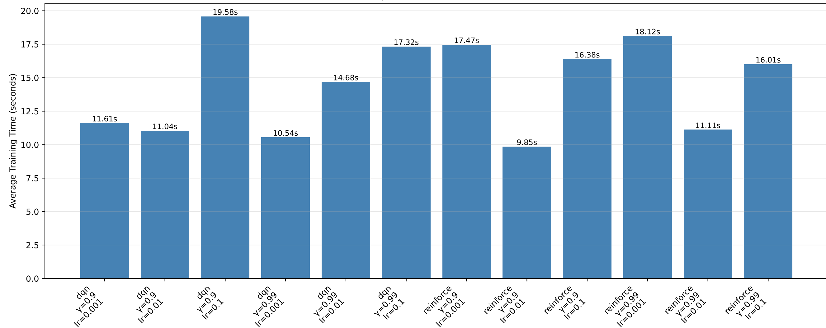
Average Runtime Across 10 Seeds
