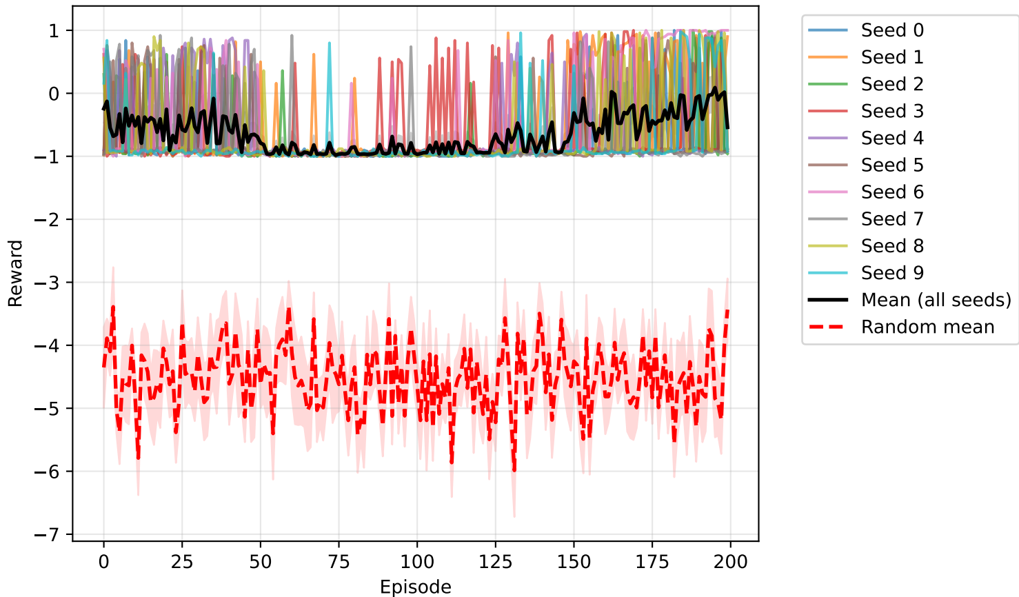
DQN Reward vs Episodes (gamma=0.9, lr=0.1)
