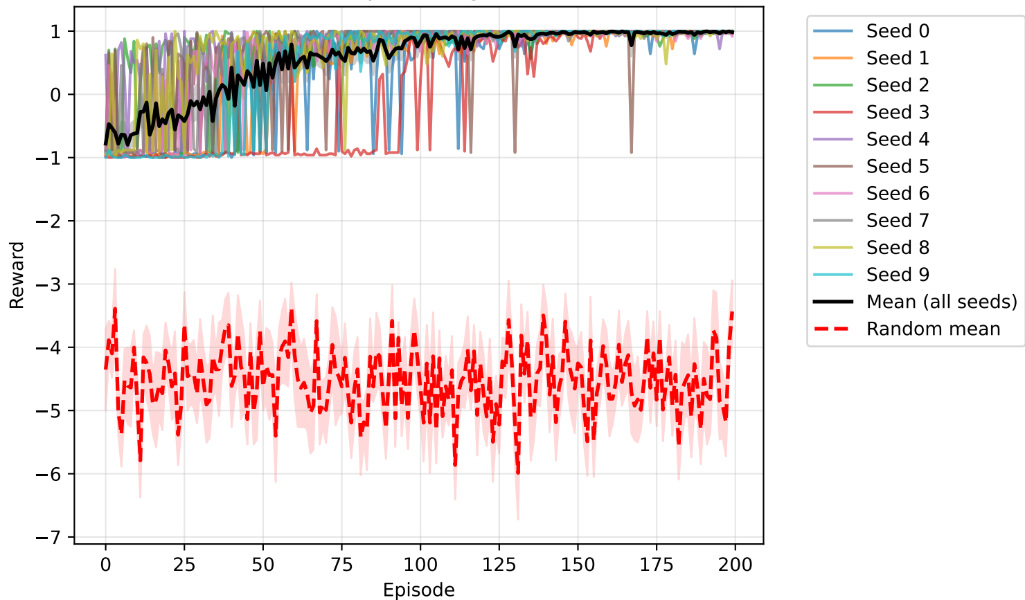
REINFORCE Reward vs Episodes (gamma=0.99, lr=0.001)
