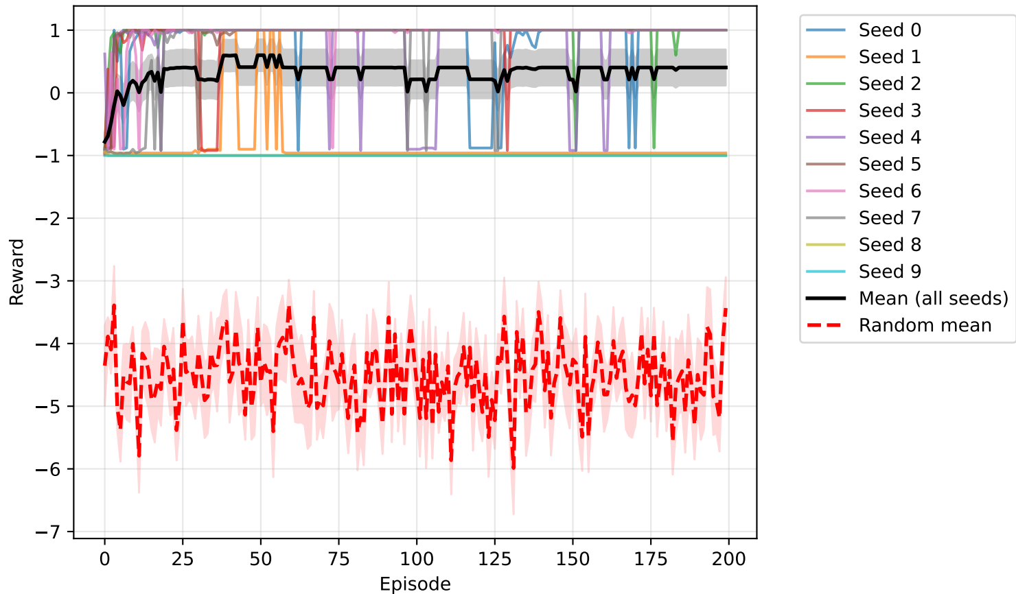
REINFORCE Reward vs Episodes (gamma=0.9, lr=0.01)
