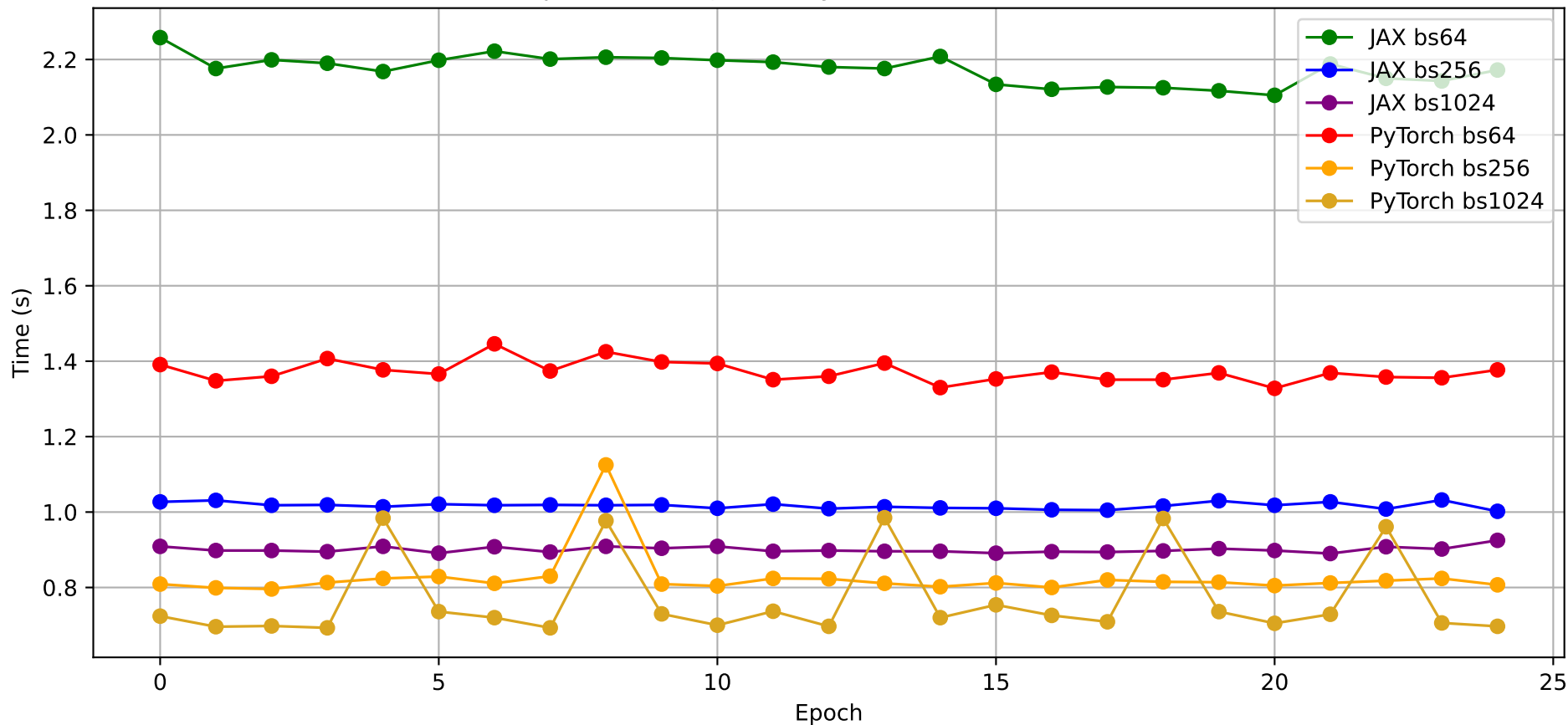
Epoch Times: JAX vs PyTorch (All Batch Sizes)
