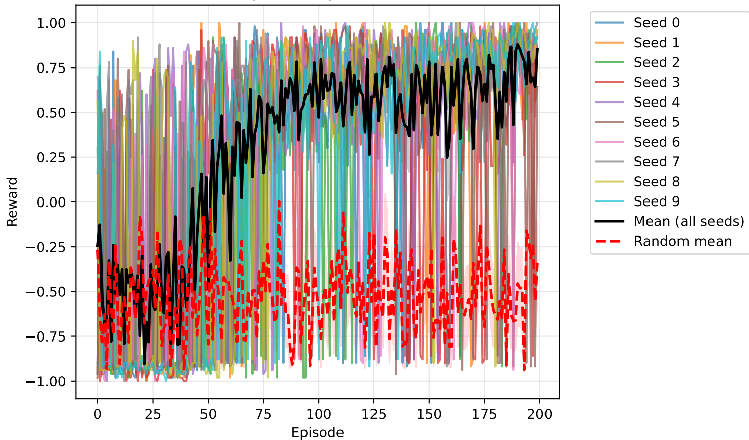
DQN Reward vs Episodes (gamma=0.99, lr=0.001)
