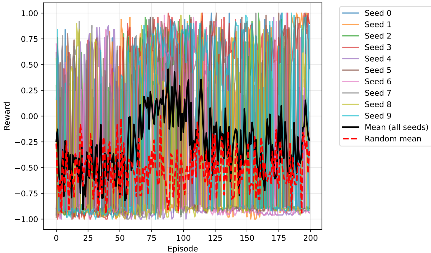
DQN Reward vs Episodes (gamma=0.99, lr=0.01)
