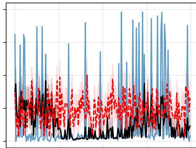
Seed 3
