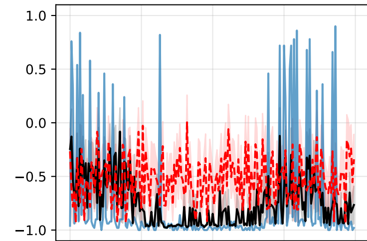
Seed 0
