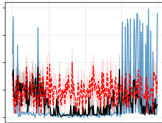
Seed 9
