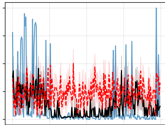
Seed 8
