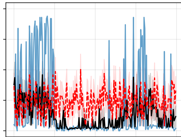
Seed 4
