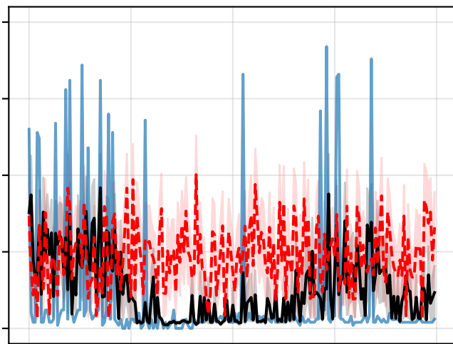
Seed 2
