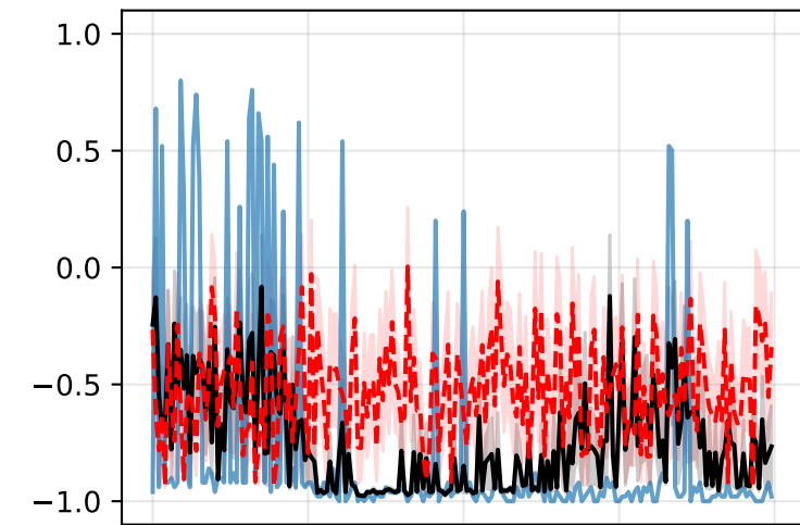
Seed 5
