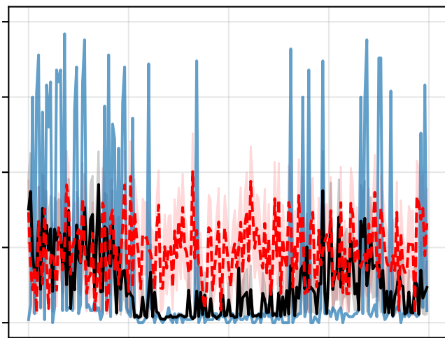
Seed 7
