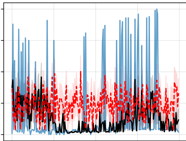
Seed 1
