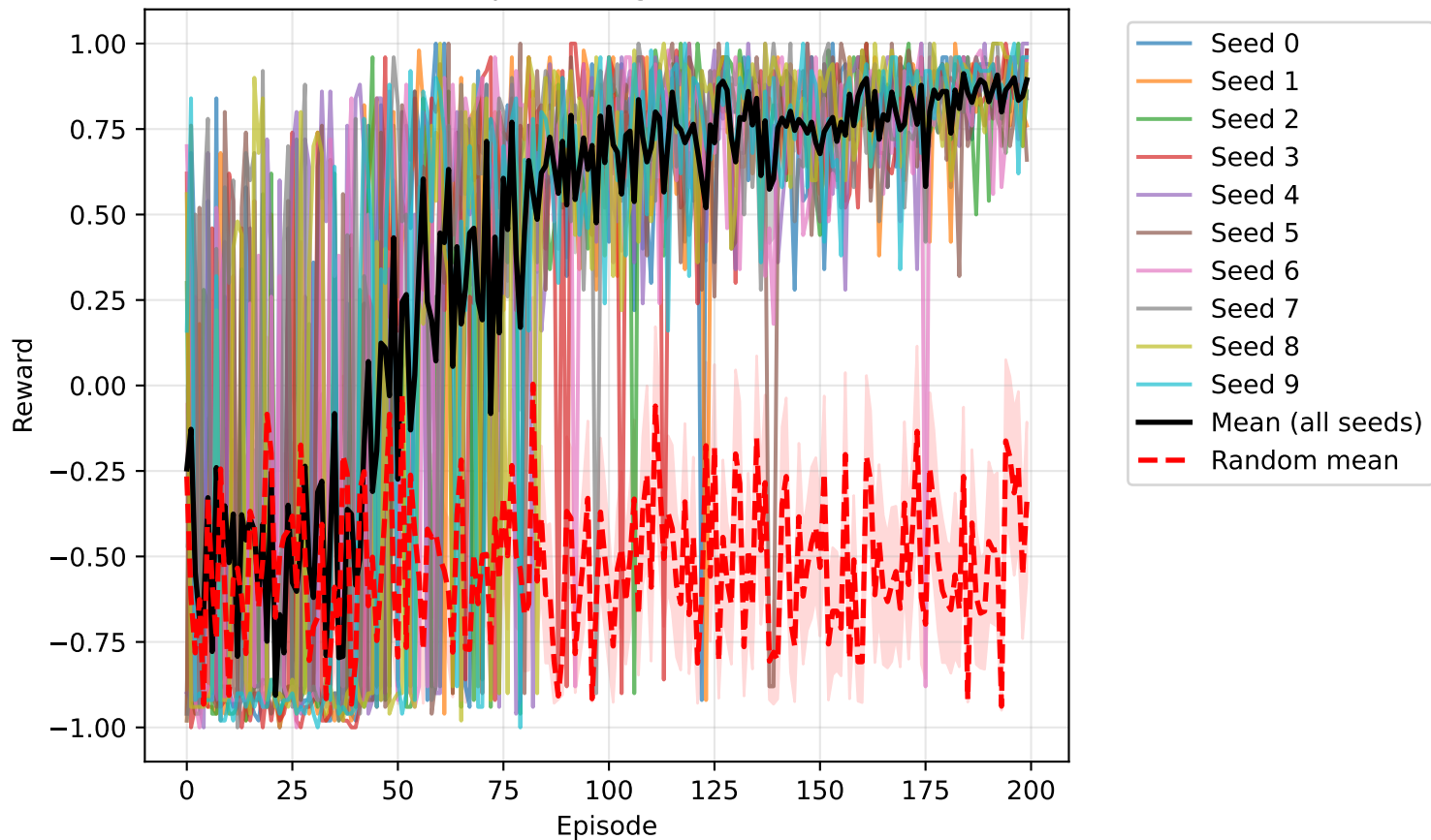
DQN Reward vs Episodes (gamma=0.9, lr=0.001)
