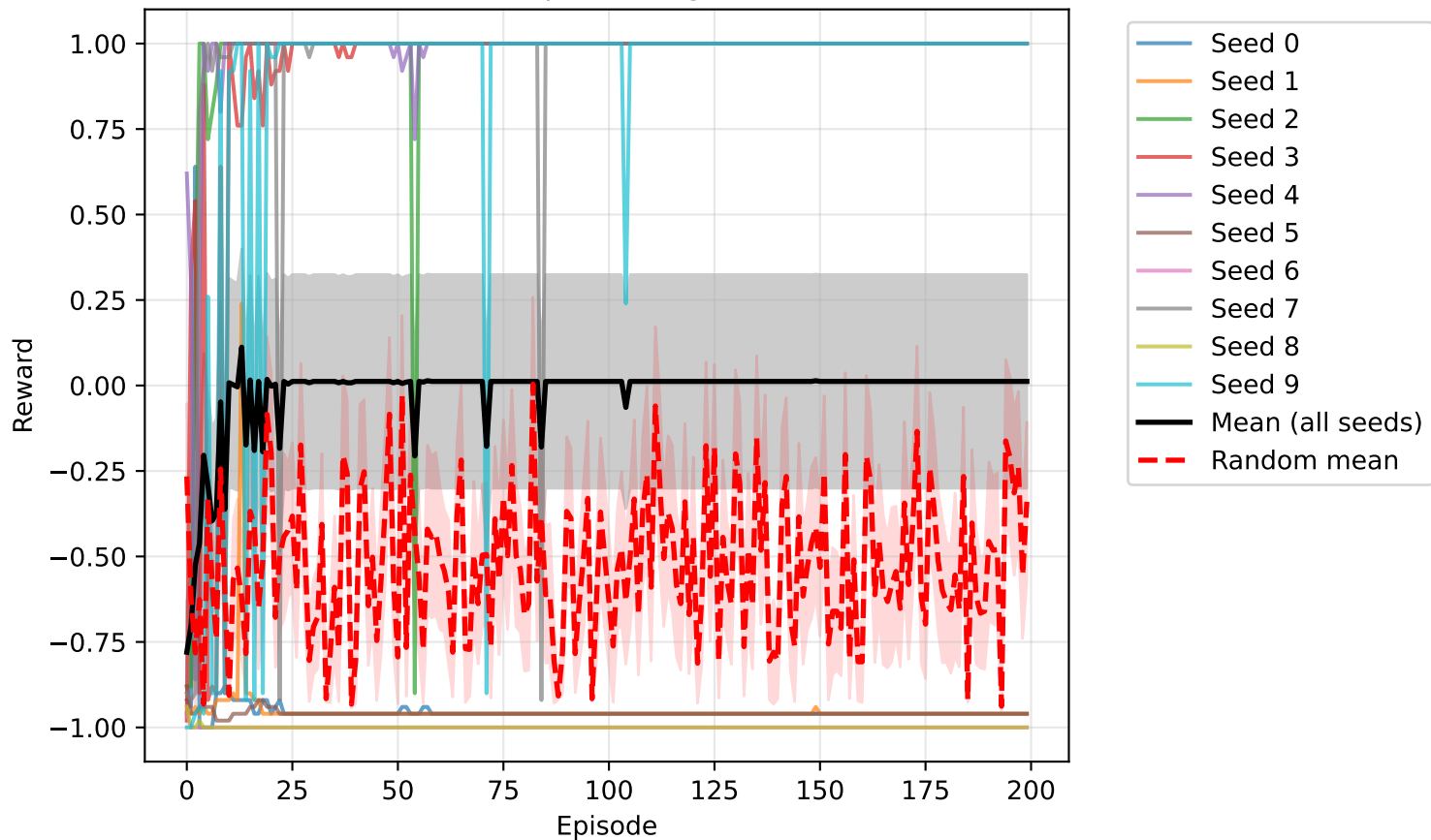
REINFORCE Reward vs Episodes (gamma=0.99, lr=0.01)
