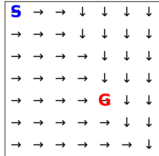
Seed 9
